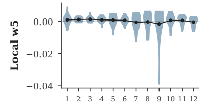
Full Shuffle
